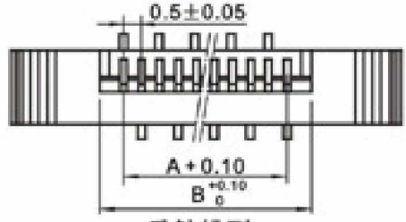
反针排列 Negative-needle arrangement
