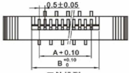
正针排列 Positive-needle arrangement
